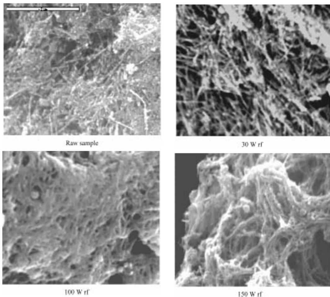
Fig. 5. SEM micrographs of the raw and the purified MWNTs with H_2S/O_2 plasmas at various rf powers.
