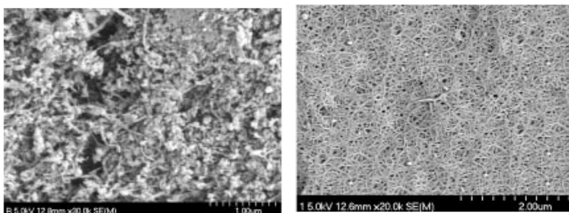
Fig. 6. SEM micrographs of the raw (left) and the purified (right) SWNTs with the combined acid treatment and H_2S-O_2 oxidation.
